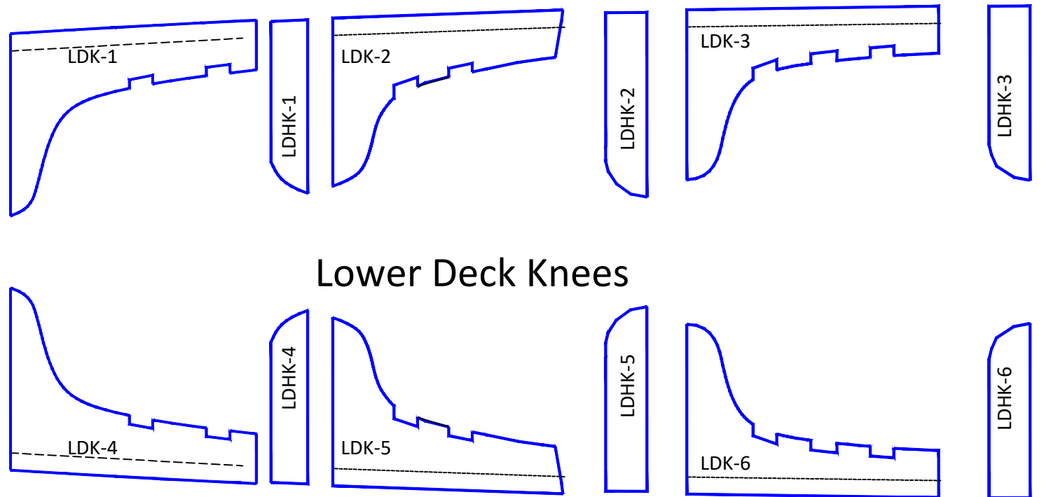
Lower Deck Framing Patterns
